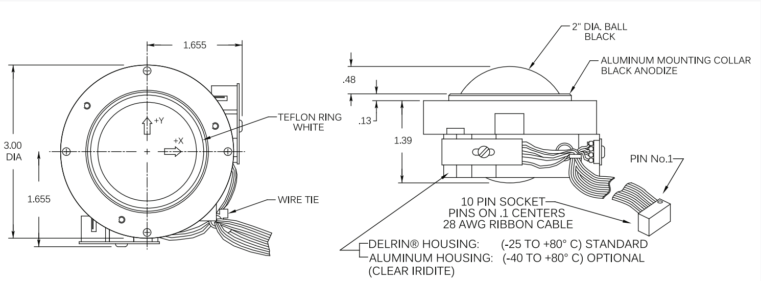
CTI Technical Drawing 761644-2 (T8XXX)
