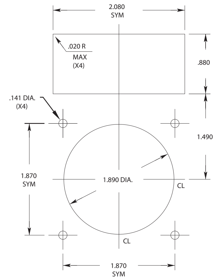
PANEL CUTOUT DETAIL
