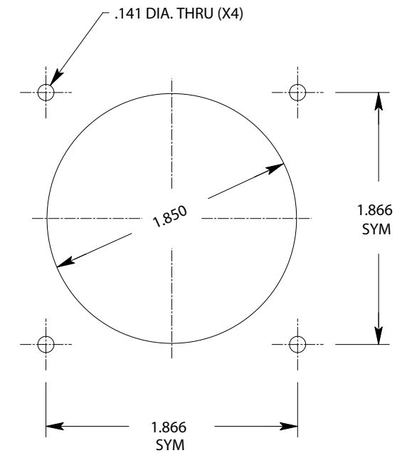
MOUNTING DETAIL
