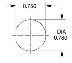
CUSTOMER PANEL CUTOUT DETAIL
