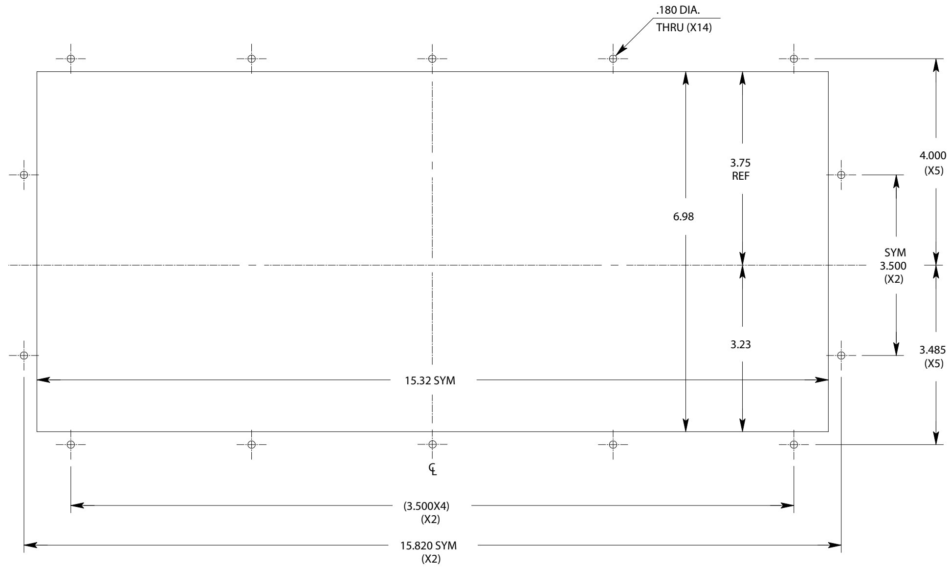
MOUNTING DETAIL
