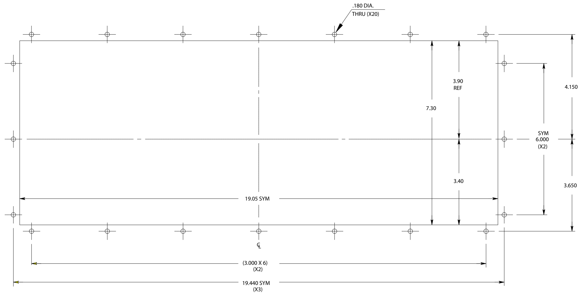
MOUNTING DETAIL
