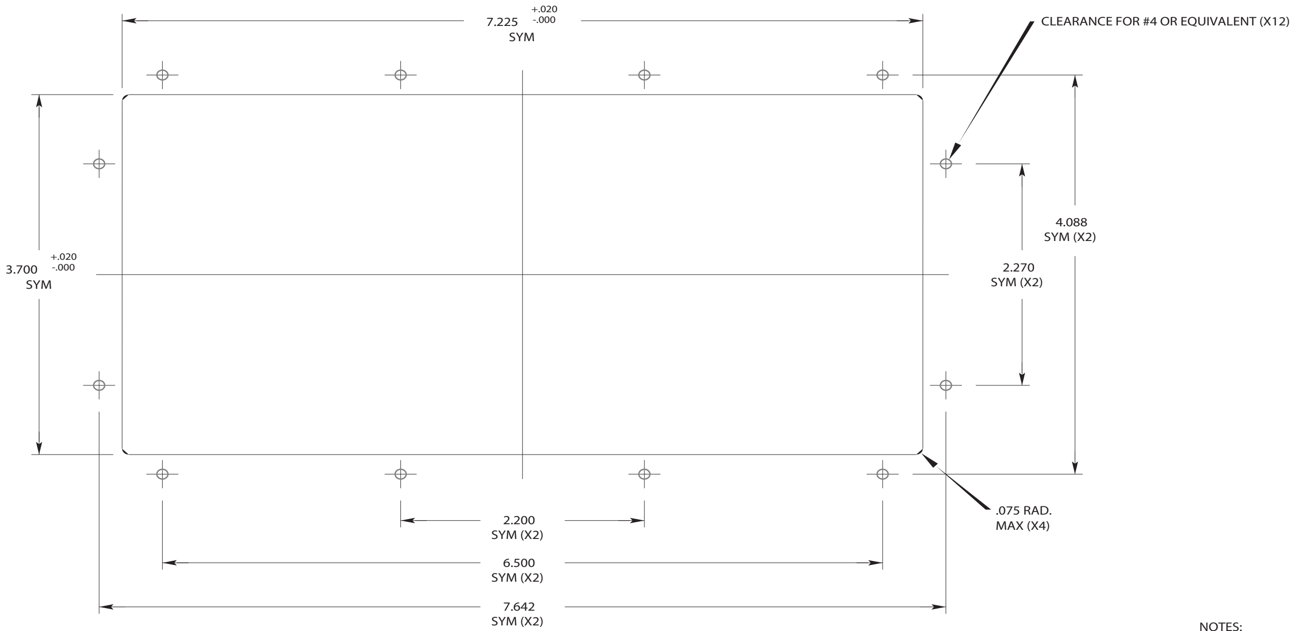
MOUNTING DETAIL
