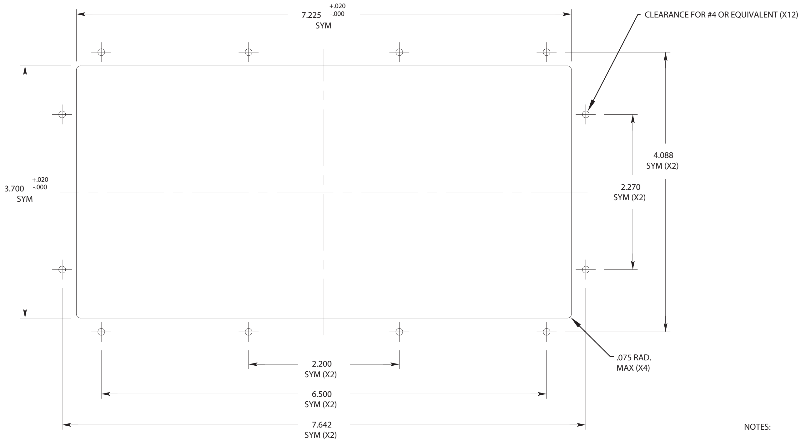
MOUNTING DETAIL
