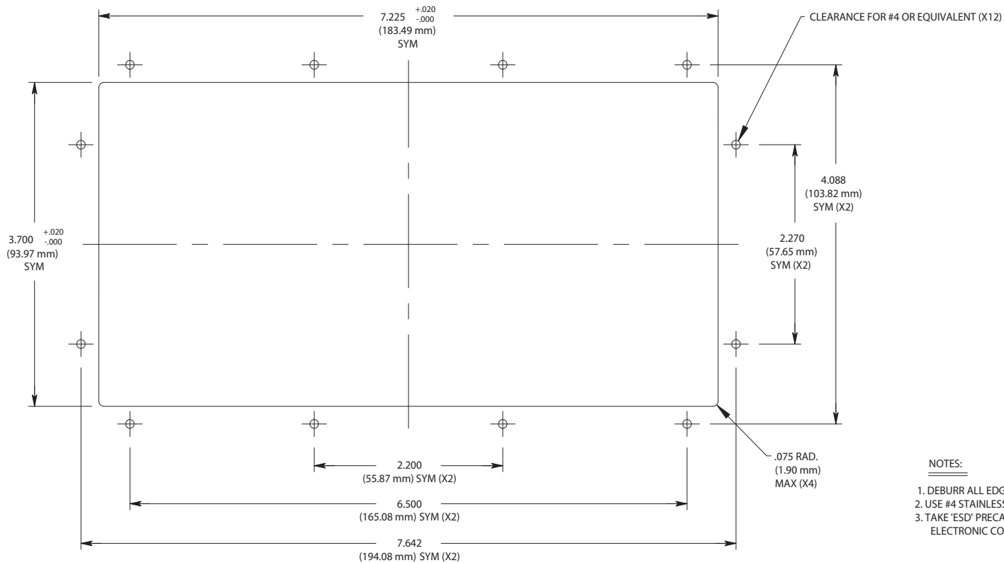
MOUNTING DETAIL
