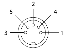
5-PIN DIN PLUG FRONT VIEW
