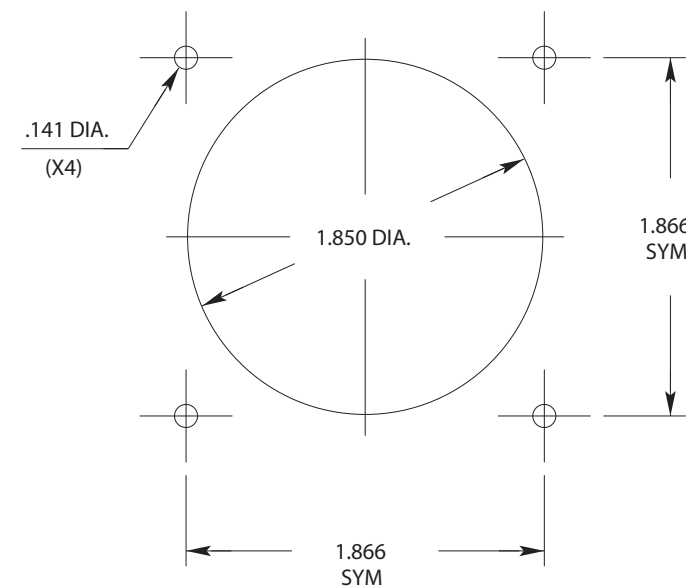
MOUNTING DETAIL
