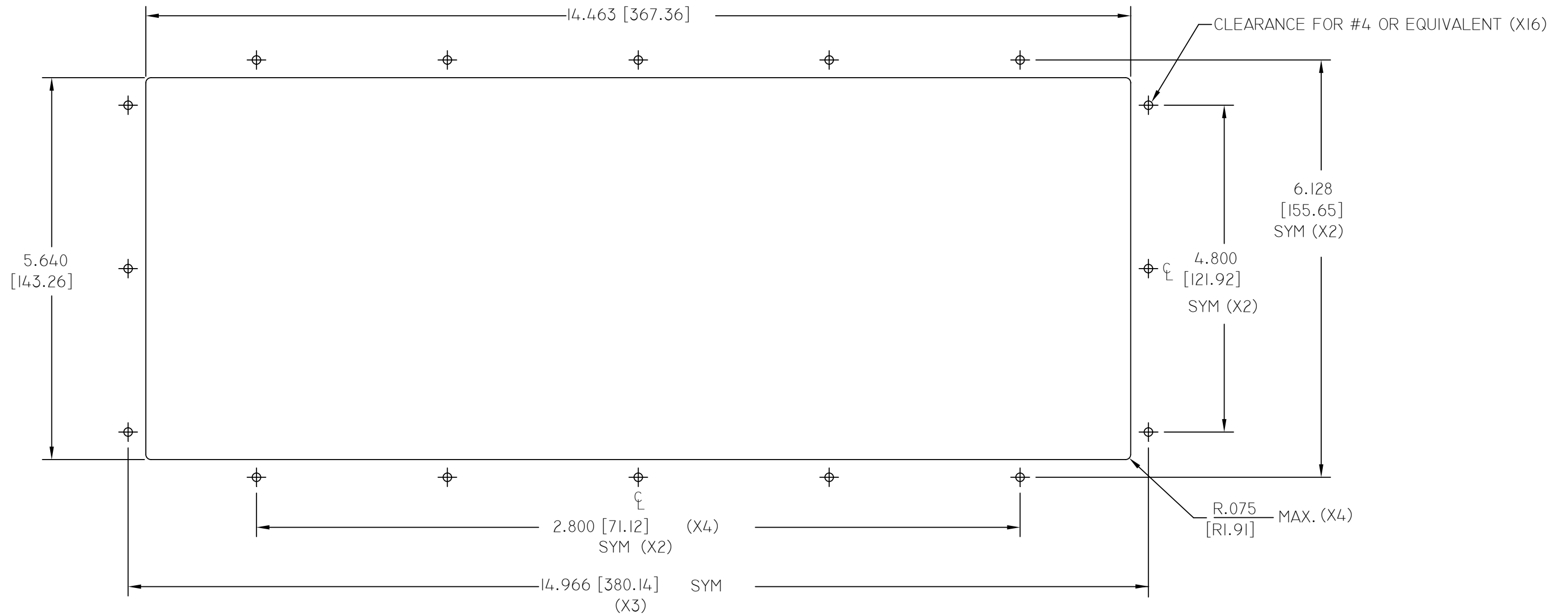
MOUNTING DETAIL
