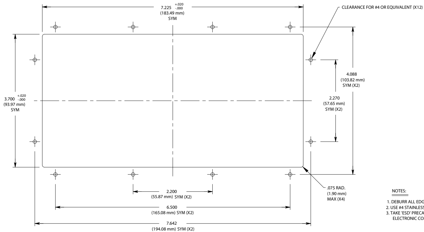
MOUNTING DETAIL
