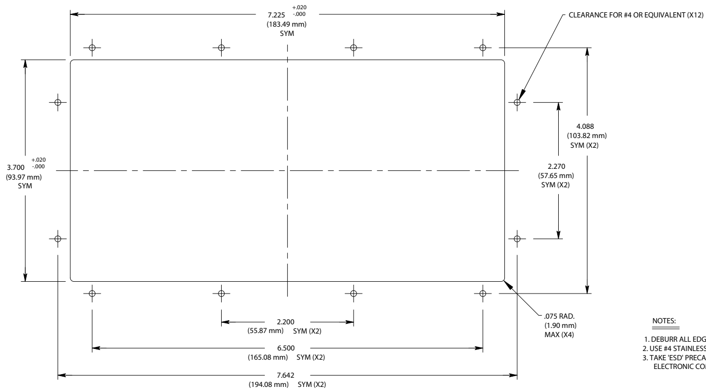
MOUNTING DETAIL
