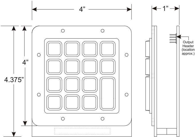
Model Number K9 Series shown (Preliminary)
