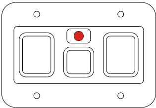
C9 Series NEMA 4 Sealed Switch Pad shown (3.3" X 2.2")
