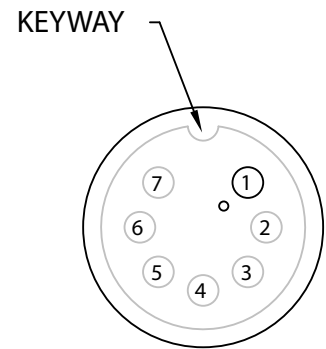
CONXALL #6282-7SG-513 FRONT VIEW
